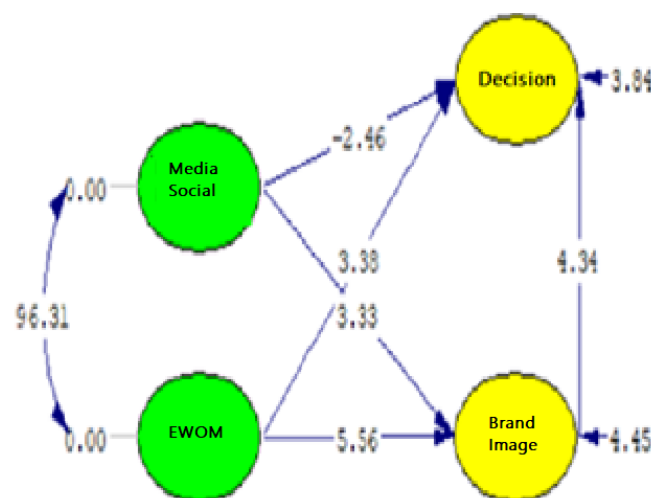
Figure 3. Tvalue Result
