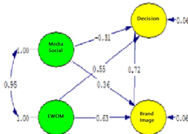
Figure 2. Standardized Result
